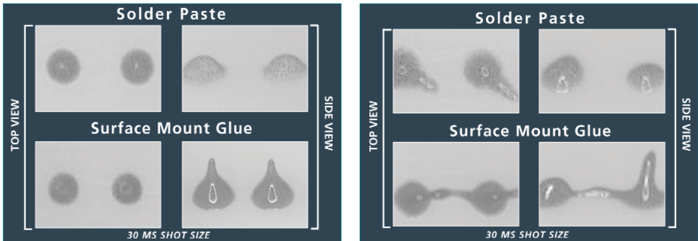
Figure 3. Dispense pattern differences, especially with adhesives, chamfered (left), non-chamfered (right).
